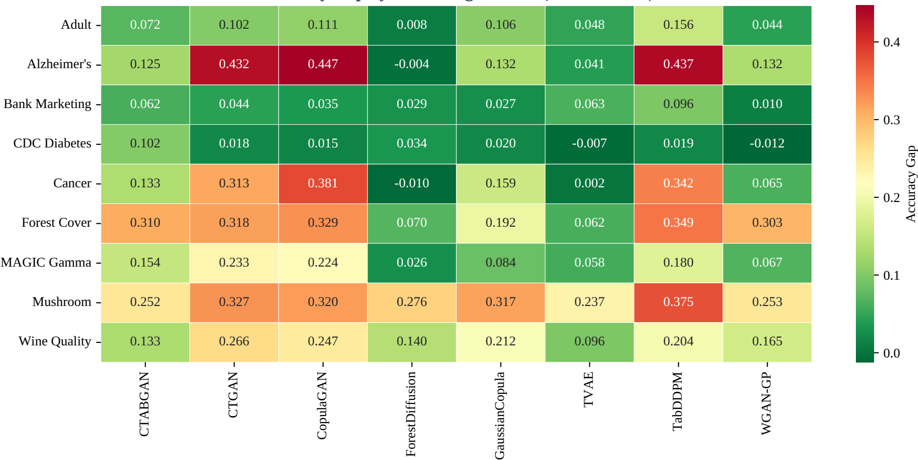
Accuracy Gap by dataset × generator (10-seed mean)
